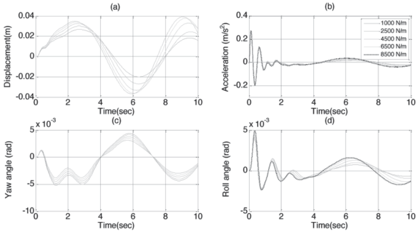
Figure 4: Effect of Secondary Lateral Spring Stiffness
