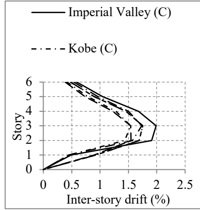
Figure 12: Inter-story drift (BRBF2)
