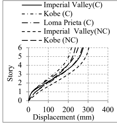
Figure 8: Story drift (BRBF2)
