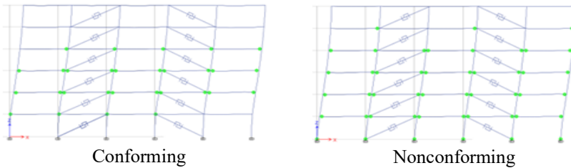
Figure 17: Plastic hinges pattern for BRBF1
