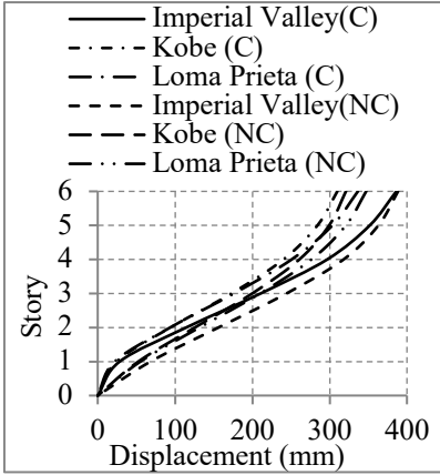
Figure 7: Story drift (BRBF1)
