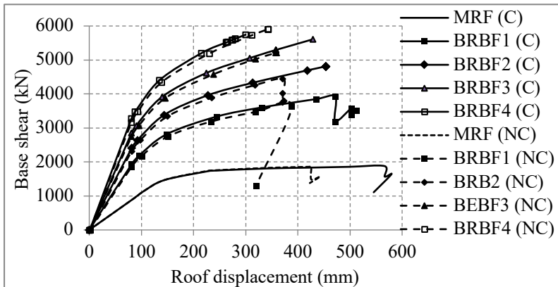
Figure 15: Capacity Curves
