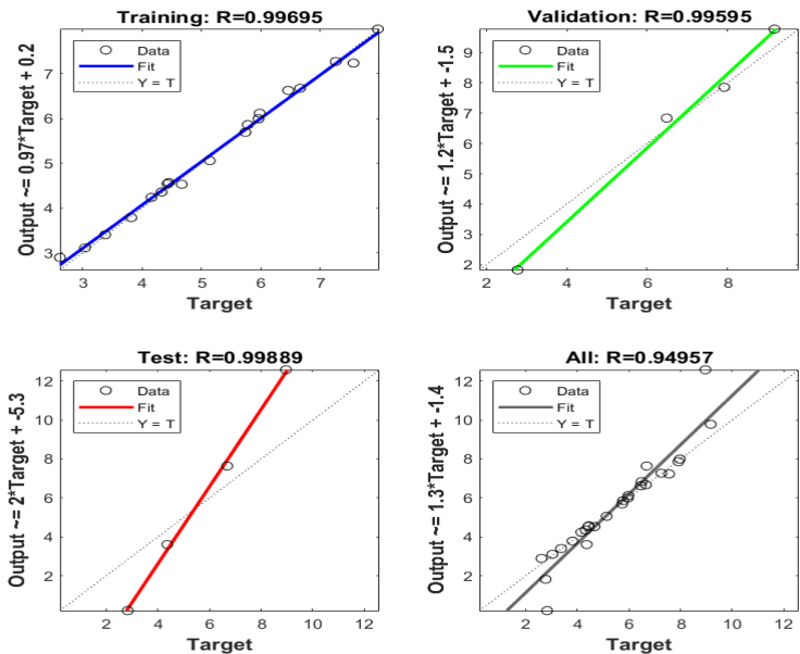
Figure 9: Coefficient of correlation (R) values for ANN.
