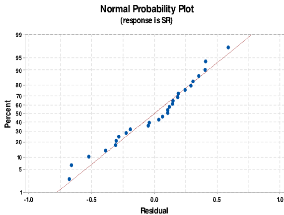
Figure 5: Normal probability of residuals for surface roughness (SR).
