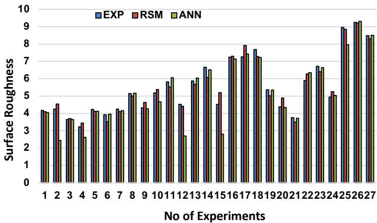
Figure10: Surface roughness values comparison graph of experimental, RSM and ANN models.
