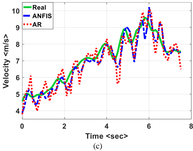
Figure 6: Velocity time series prediction based on ANFIS and AR models, (a) 0.1 second ahead, (b) 0.2 second ahead, (c) 0.3 second ahead.
