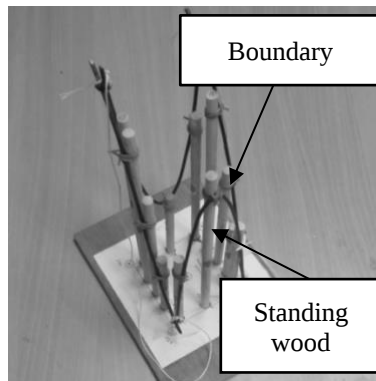
Figure 3: Soap Film Model with standing wood and boundary.
