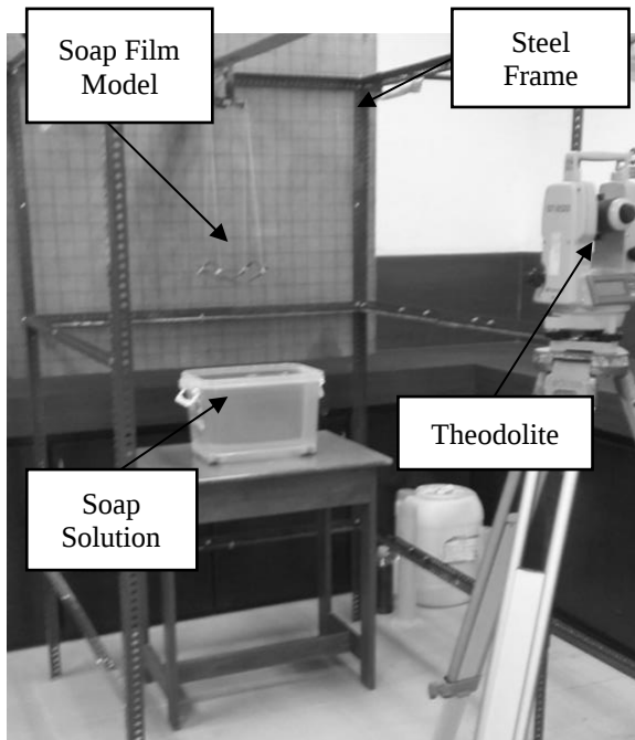
Figure 4: Experiment setup for soap film model.
