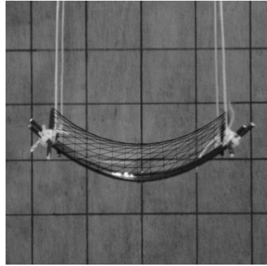
Figure 6 : Comparison of experimental and computational results of Handkerchief Surface, u=v=0.2
