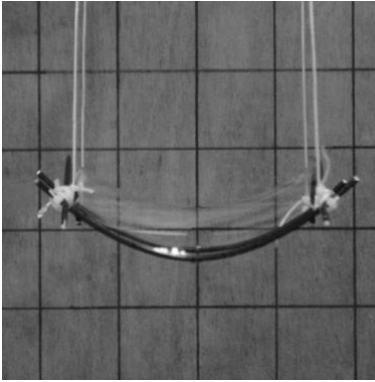
Figure 5 : Soap film model of Handkerchief Surface, u=v=0.2
