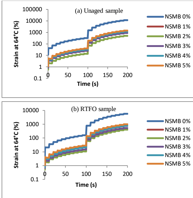
Figure 8: MSCR result at temperature of 64°C, (a) unaged sample (b) RTFO sample
