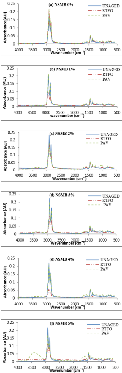
Figure 3: FTIR spectra of NSMB
