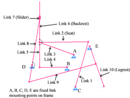
Figure 3: The kinematic concept of a reconfigurable wheelchair
