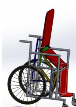
Figure 5: Wheelchair at standing configuration
