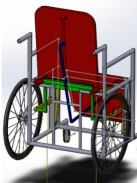
Figure 4: Linkage structure with frame for seat position
