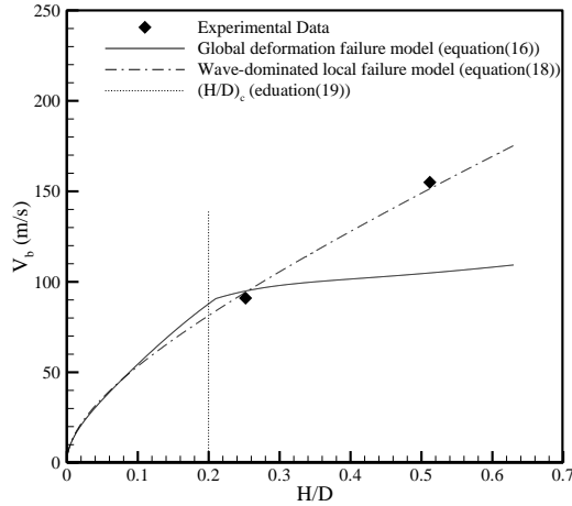
Figure 4: Comparison between ballistic limit velocity obtained from represented model and experimental data in reference [5]
