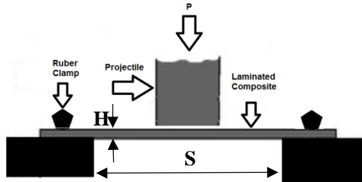
Figure 1: Laminated plate encountering a flat head projectile impact.
