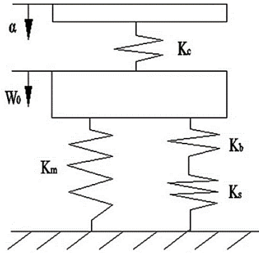
Figure 2: Impact spring model
