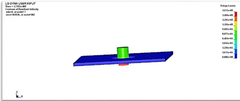
Figure 9: 4.5mm thick E-glass/epoxy laminate perforated by a projectile.
