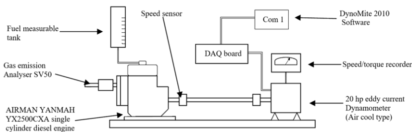
Figure 1: Schematic diagram for engine performance testing setup
